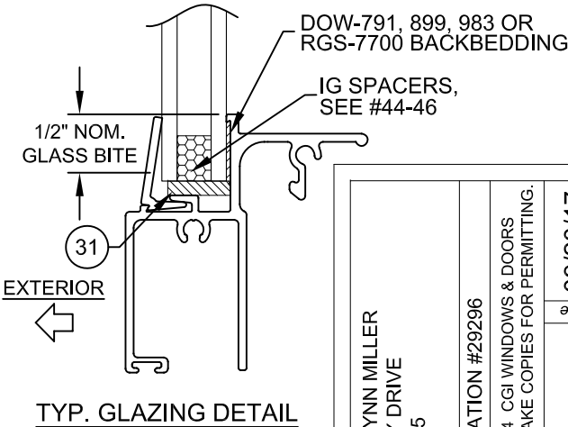
TYP. GLAZING DETAIL
