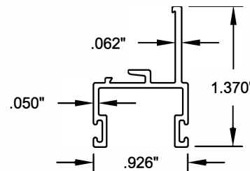
10 SASH SIDE RAIL 6063-T6 ALUMINUM
