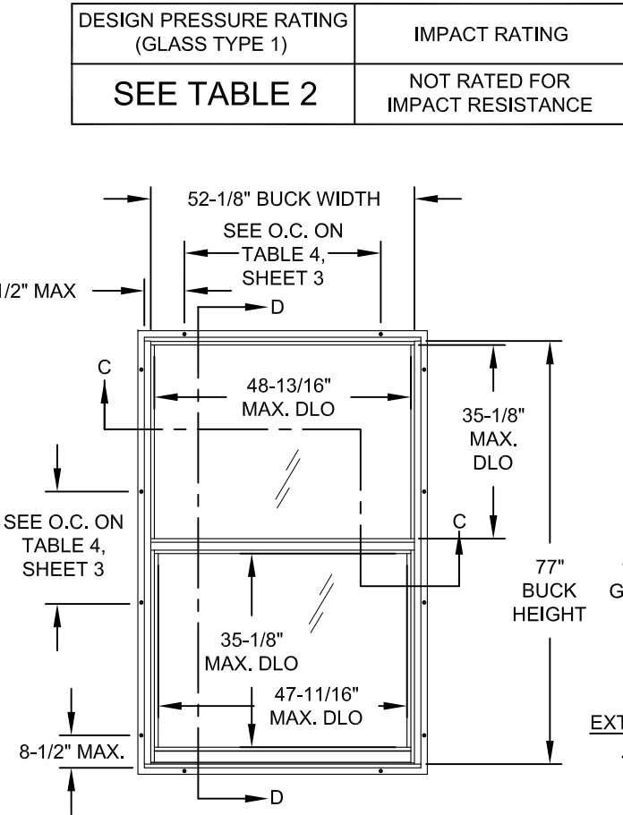
TYP. INTEGRAL FIN FRAME ANCHOR LOCATIONS @ MAX. SIZE (INSTALLED WITH SCREWS)
