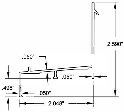
2 FLANGE FRAME SILL 6063-T6 ALUMINUM
