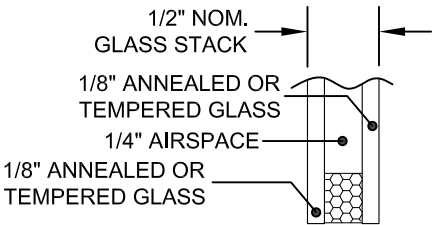
1/2" I.G. GLAZING GLASS TYPES 7 & 9
