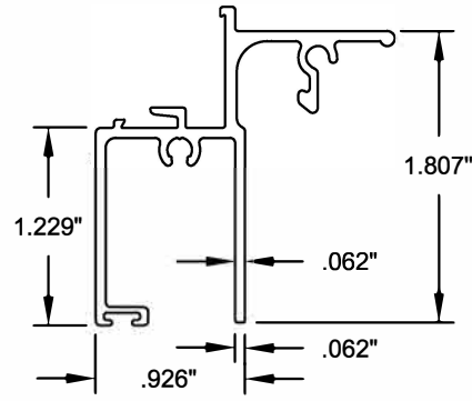
7 SASH BOTTOM RAIL 6063-T6 ALUMINUM
