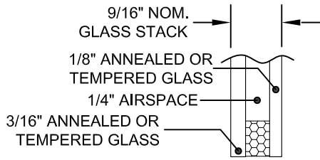
9/16" I.G. GLAZING GLASS TYPES 8 & 10
