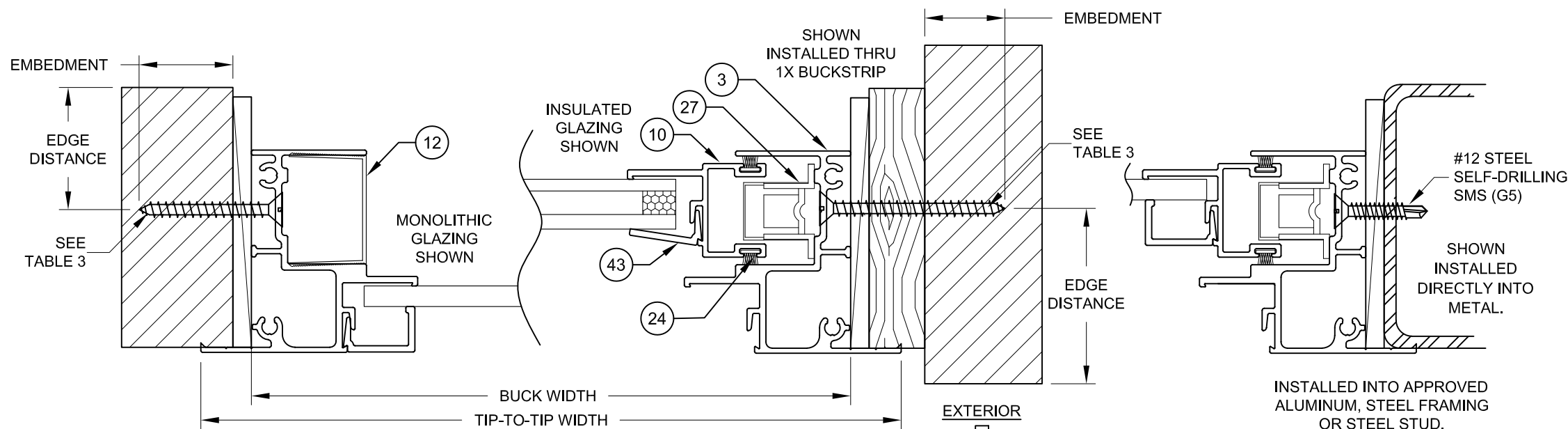
HORIZONTAL SECTION A-A
