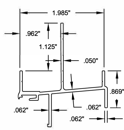
4 INTEGRAL FIN FRAME HEAD 6063-T5 ALUMINUM
