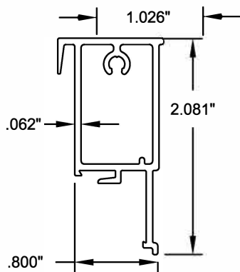
8 SASH TOP RAIL 6063-T6 ALUMINUM
